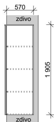
Bokorys
