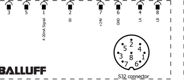
=+20HHL21 CG001 -B01 +20CBB01/81.2:E Micropulse Transducer - Rod Style BTL7-E100-M1200-B-S32
