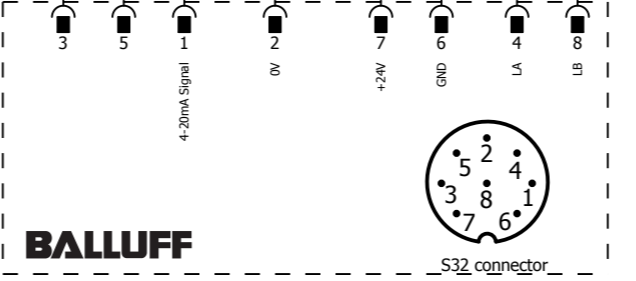
=+20HHL22 CG003 -B01 Micropulse Transducer - Rod Style BTL7-E100-M0200-B-S32
