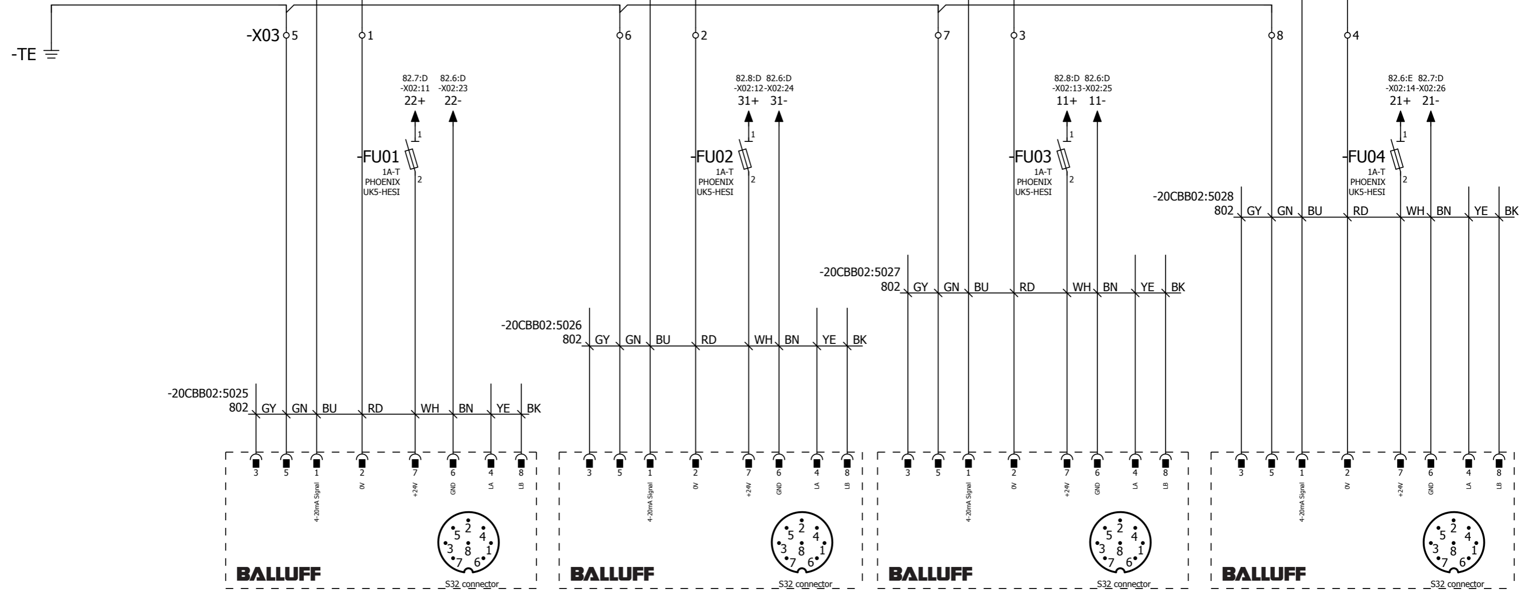
=+20HHL22 CG002 -B01 Micropulse Transducer - Rod Style BTL7-E100-M0200-B-S32
