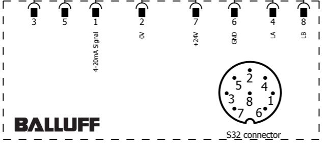
=+20HHL22 CG002 -B01 Micropulse Transducer - Rod Style BTL7-E100-M0200-B-S32
