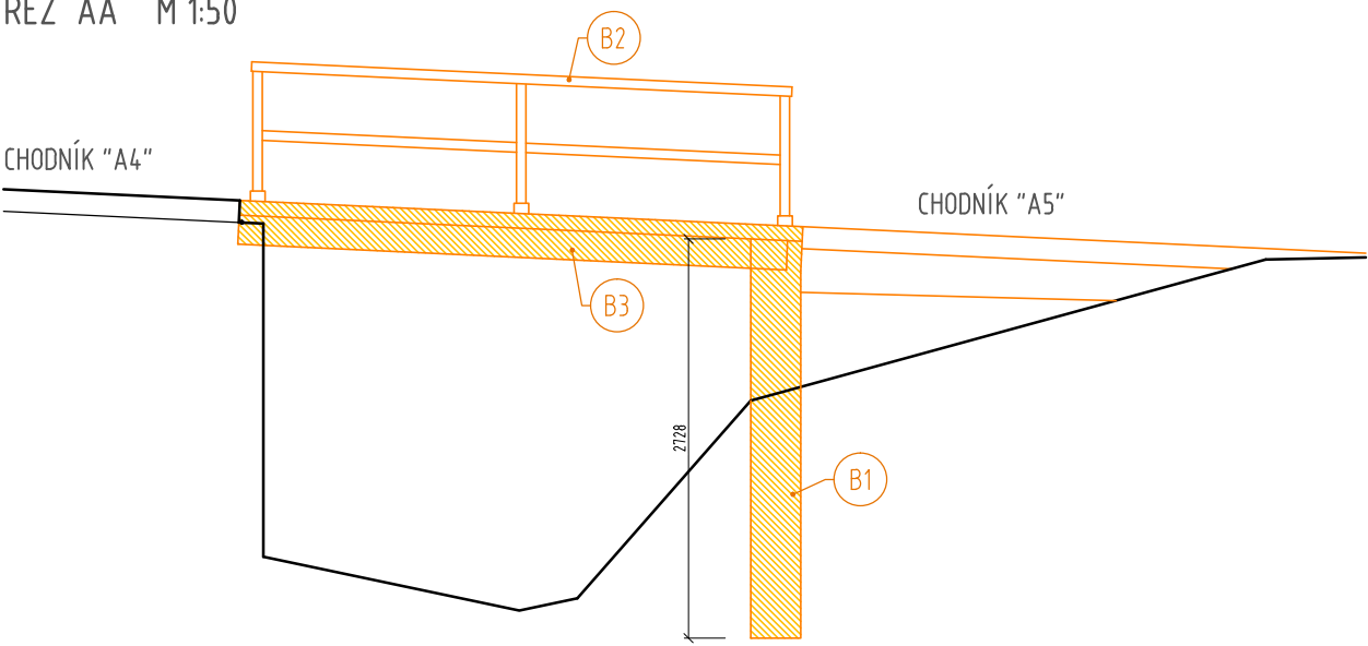
REZ AA M 1:50
