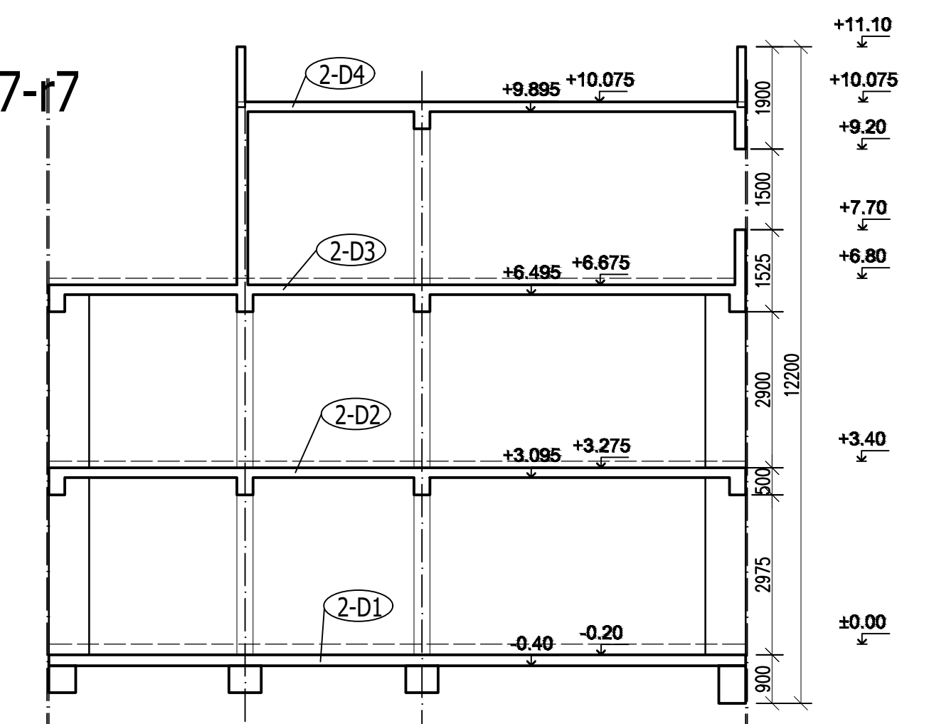
REZ r8-r8 M 1:100
