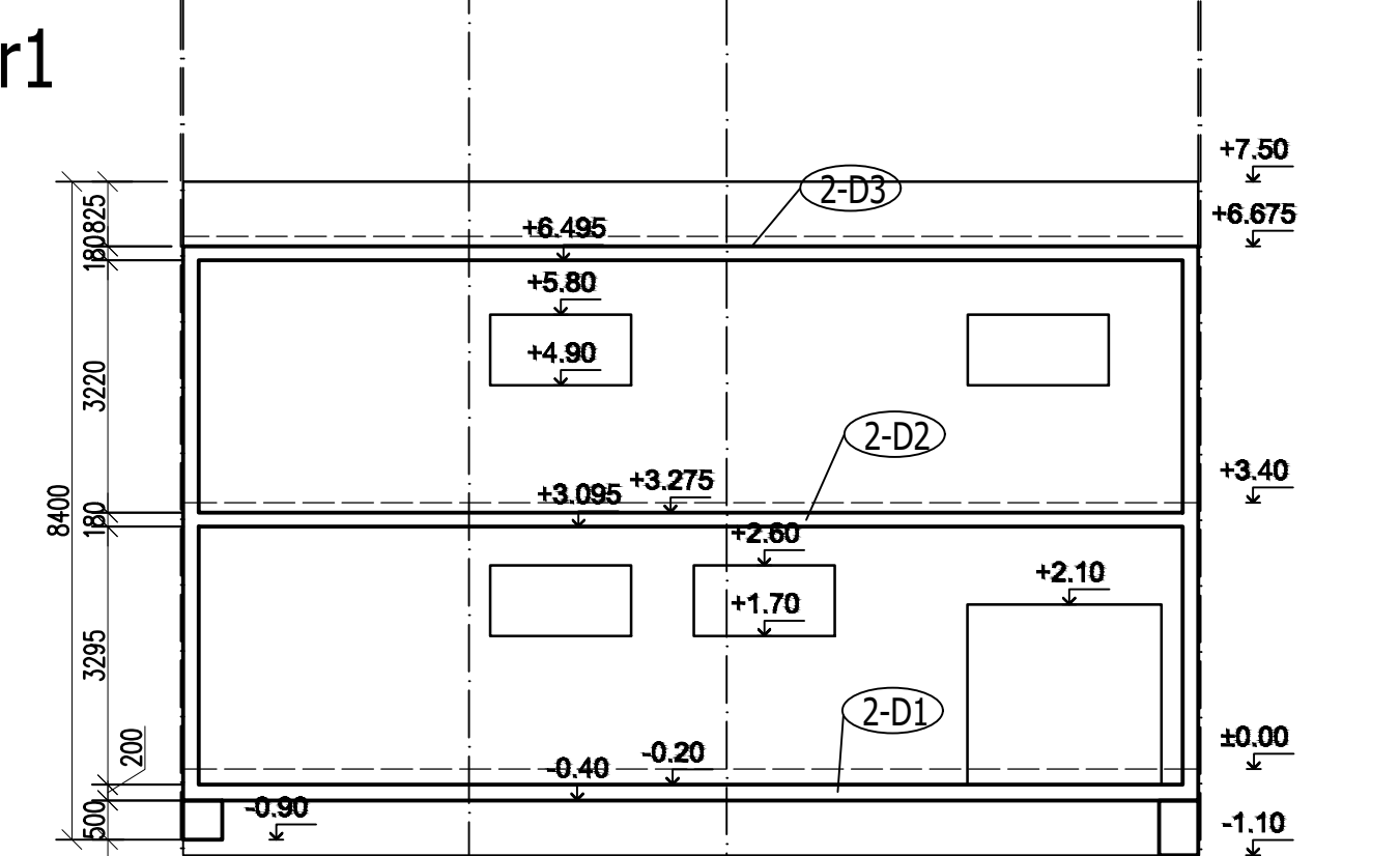
REZ r2-r2 M 1:100
