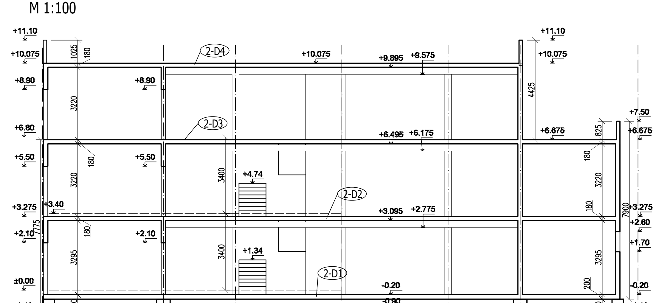
REZ r13-r13 M 1:100
